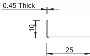
Ceiling Angle
