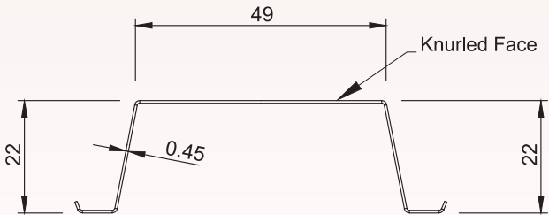
Ceiling Section
