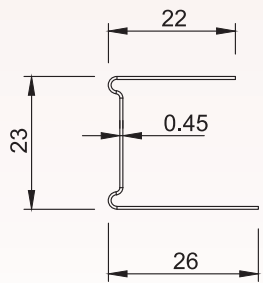
Perimeter Channel
