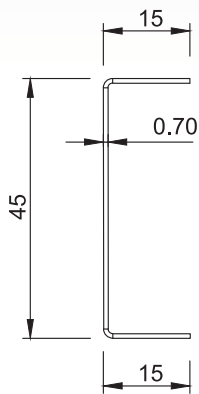
Intermediate Section
